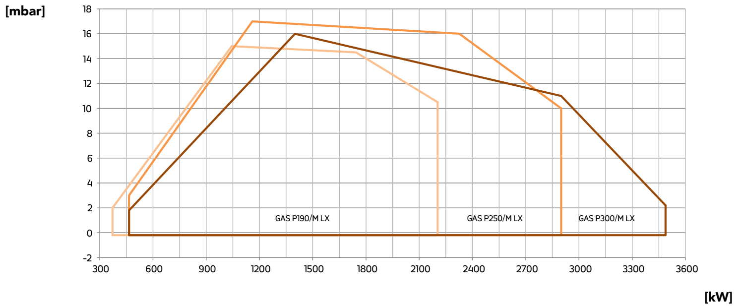
Fig. 2 X = Thermal power [kW] Y = Pression in the combustion chamber [mbar]
