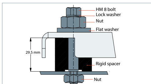
Rigid spacers to remove
