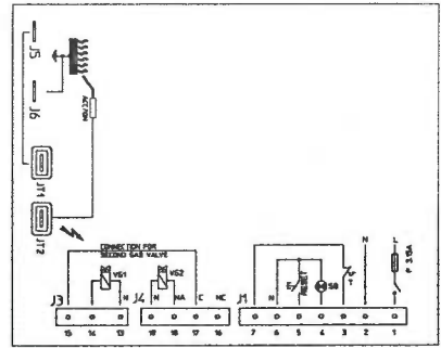
TYPE MM51F
