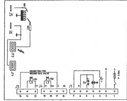
TYPE SM11F
