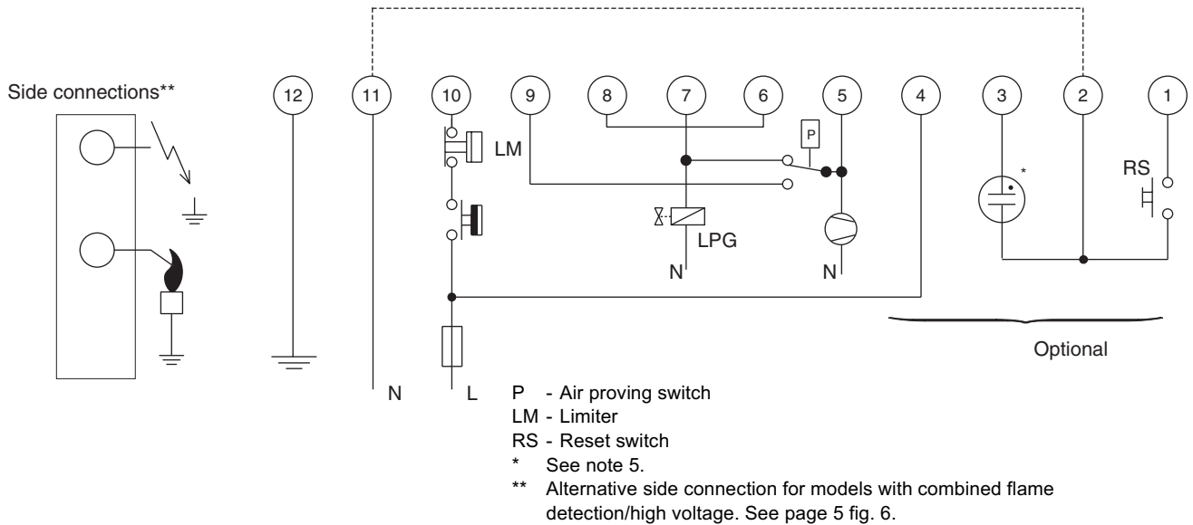
Fig. 5. Connection diagram S4565C, D, R, T
