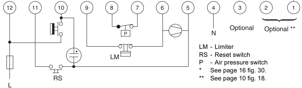
Fig. 25. Connection diagram S4565CD and DD "2000" series
