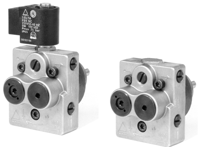
A AD Oil burners fuel unit
